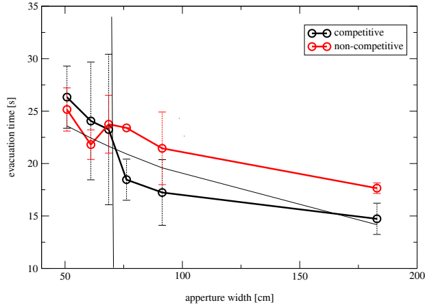
Fig. 3.20. The evacuation time increases with decreasing aperture width. For non-competitive situations, this decrease is rather smooth. However, if there is competition, at a certain aperture width ( w_c \approx 70 cm) the increase in the egress time is quite drastic and the performance is worse than in the case of non-competition [Muir, 1996].
