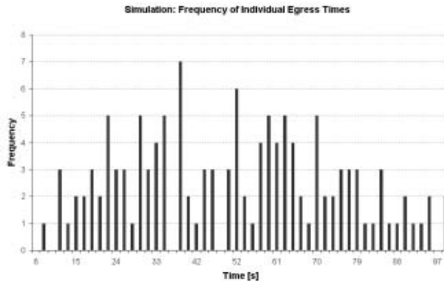
Fig. 4.12. Individual egress times obtained for the simulation.
