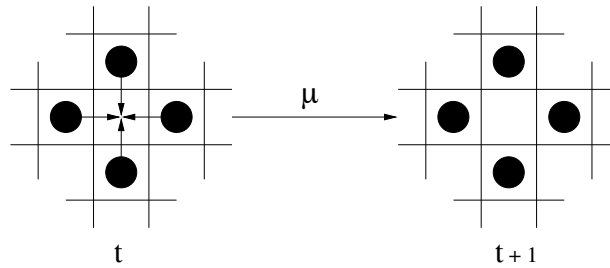
Fig. 3.21. Illustration of the friction concept and the parameter \mu . For \mu = 1 there is no winner in a conflict, for \mu = 0 , friction is turned off.
